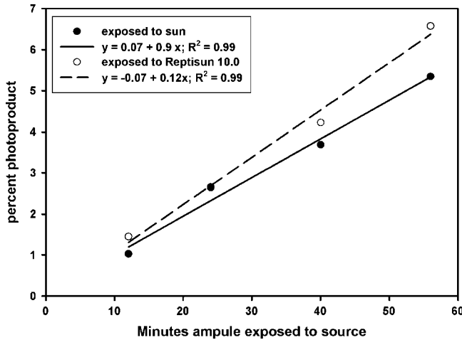
Fig. 7. Percent photoproduct in ampules vs. time exposed to sunlight or an artificial UVB source (20 Watt ZooMed Reptisun 10.0 fluorescent tube). Each ampule was exposed to the same average irradiance (43 IU/min) measured with the Solartech 6.4 m. There were no significant differences in slope or intercept of the regressions for the sun vs. the Reptisun tube (see text).
