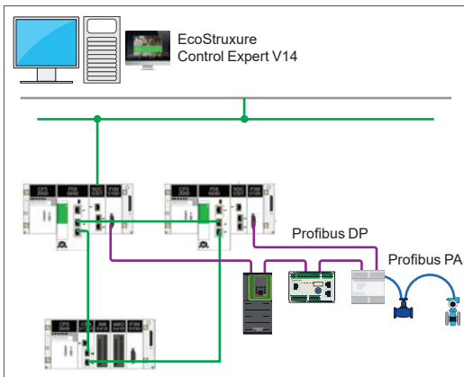
Redundant (HSBY) topology to connect the Profibus DP master X80 module to M580/X80 platforms with PMPXM0100
