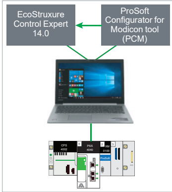
Interaction between EcoStruxure Control Expert, Prosoft Configurator for Modicon (PCM tool), and PMPXM0100 Profibus DP master X80 module
