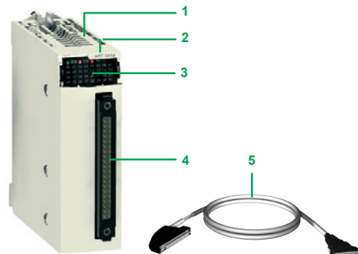
Module for connection via 40-way connector
