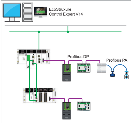
Standalone topology to connect Profibus DP master X80 module to M580/X80 platforms with PMPXM0100
