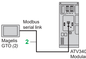
Example of connecting a modular ATV340 drive to a Magelis GTO HMI terminal via the Modbus serial link
